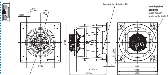
K3G 500-PB33-01 (Centrifugal module with support bracket)
